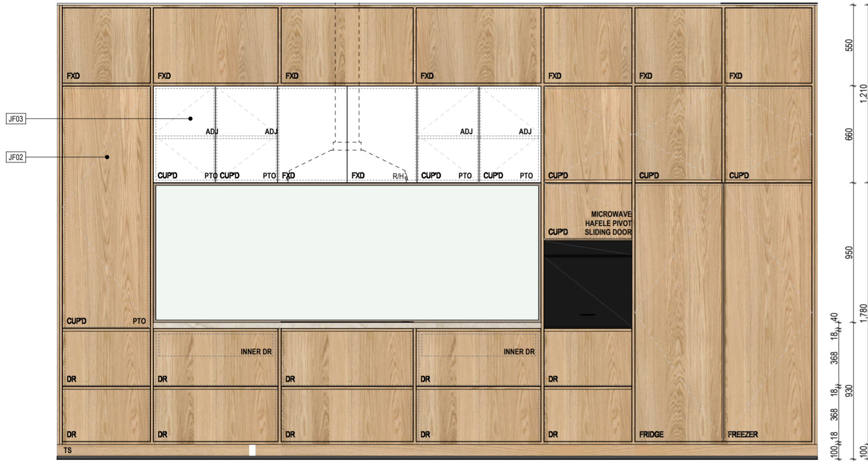
01 Back Wall Elevation
