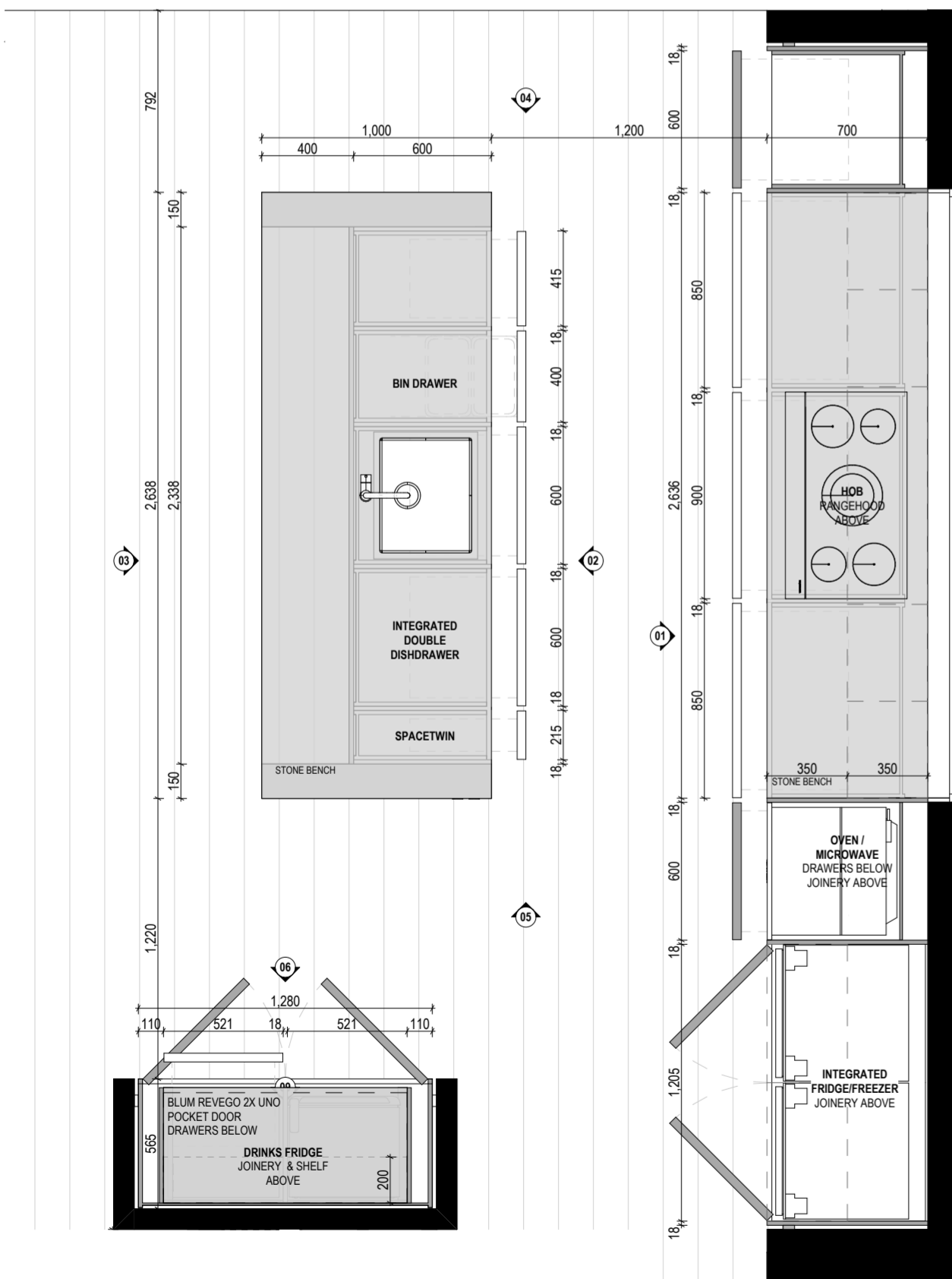
Kitchen Plan
