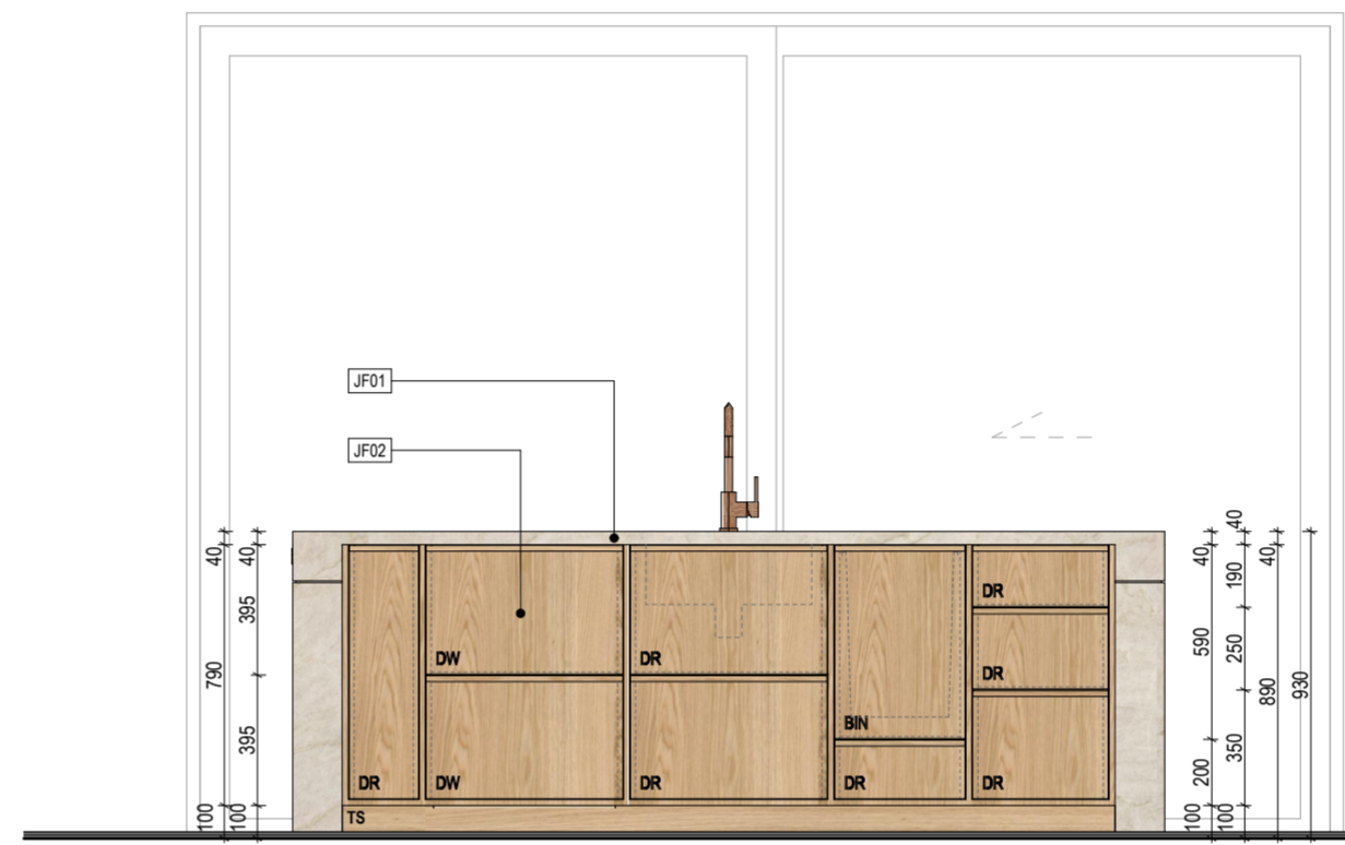
02 Island Back Elevation
