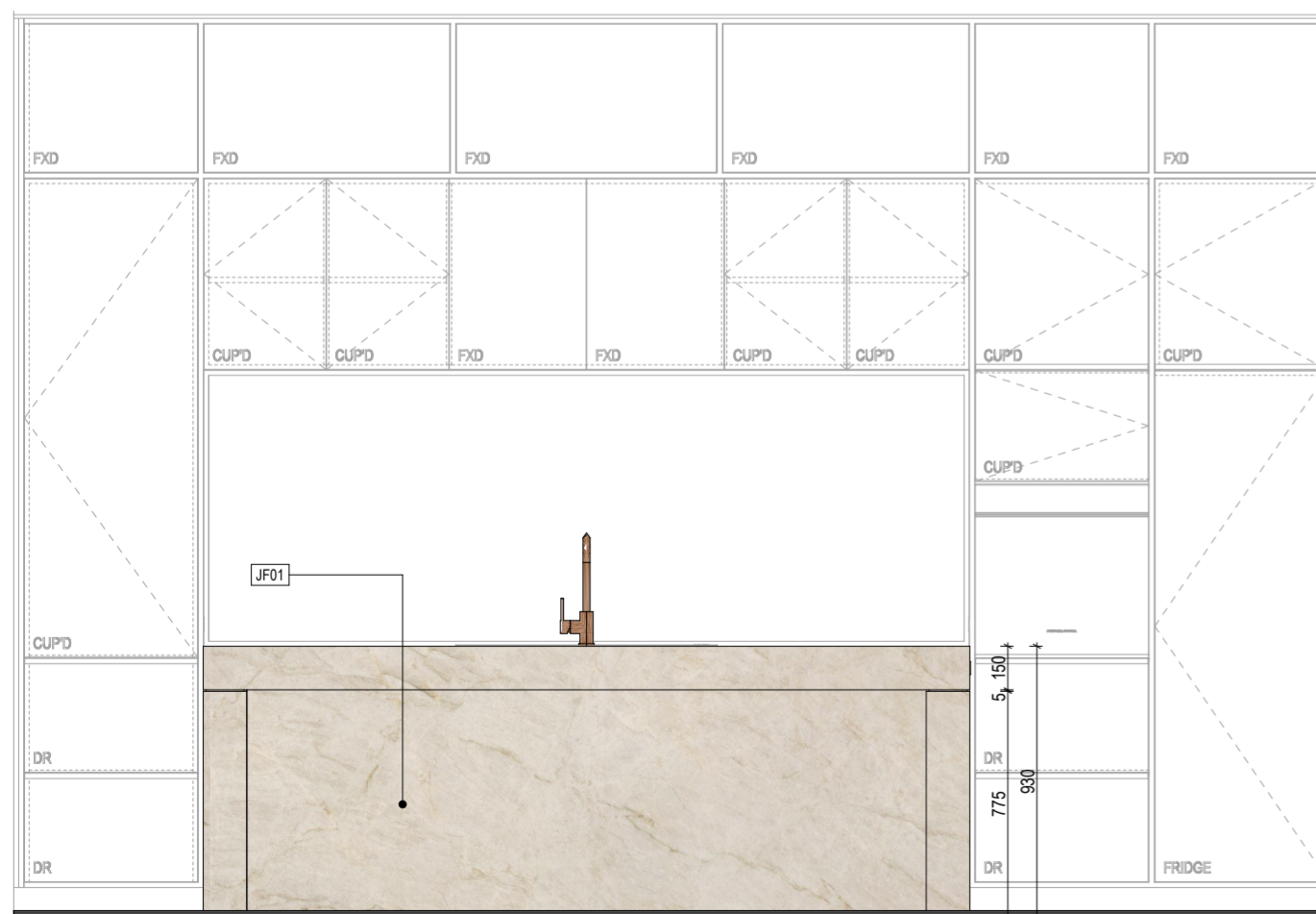
03 Island Front Elevation
