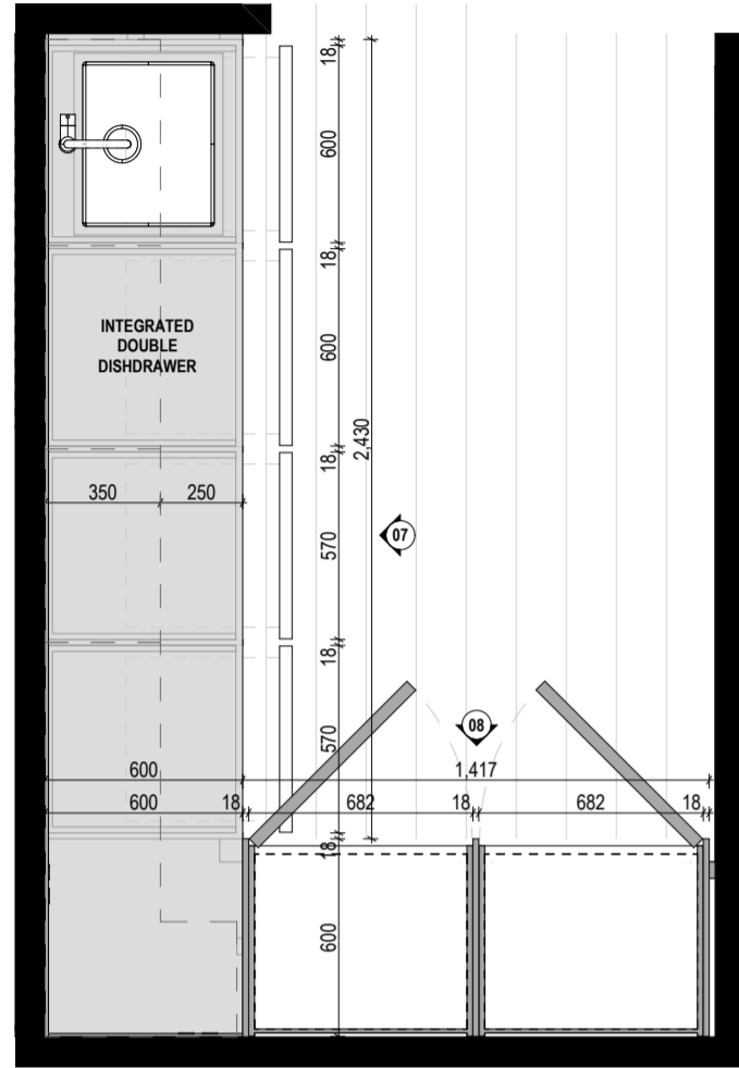
Kitchen Plan SCALE: 1:25
