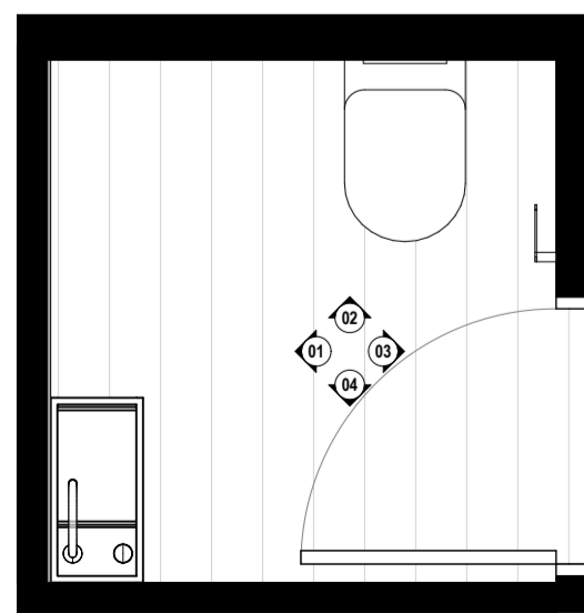
Powder Room Plan SCALE: 1:25
