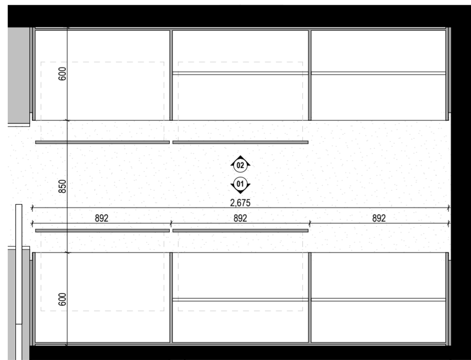
Walk In Robe Plan SCALE: 1:25
