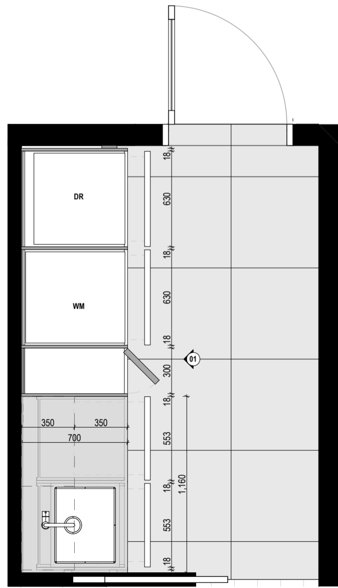
Laundry Plan SCALE: 1:25
