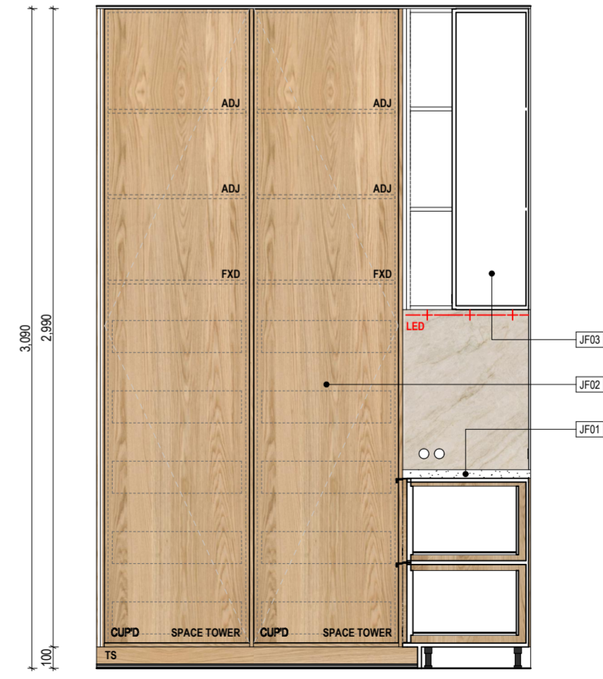
09 Scullery Elevation
