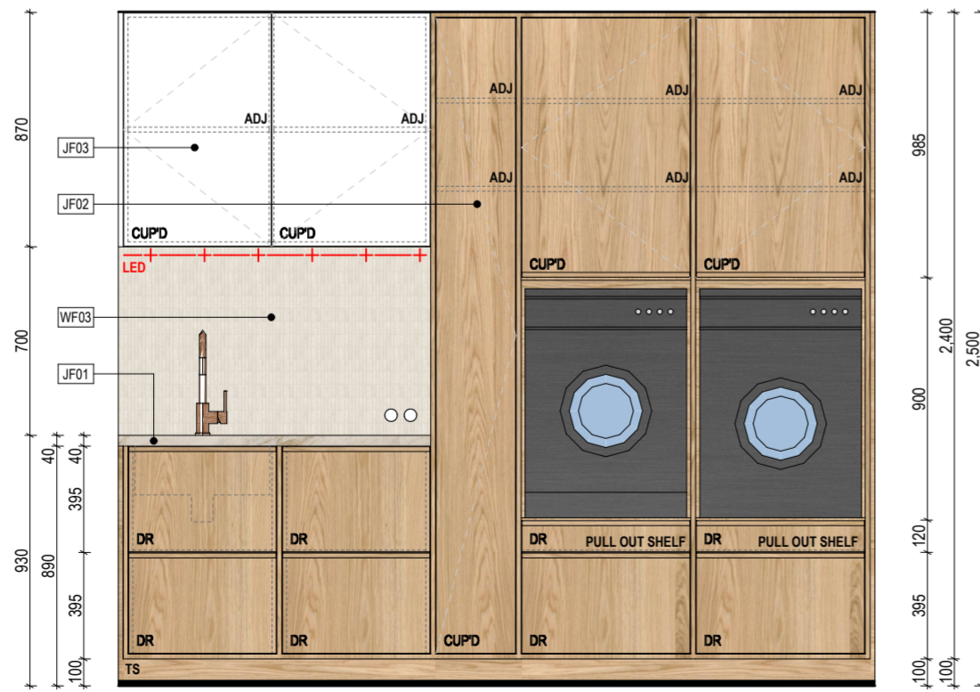
01 Laundry Elevation SCALE: 1:25
