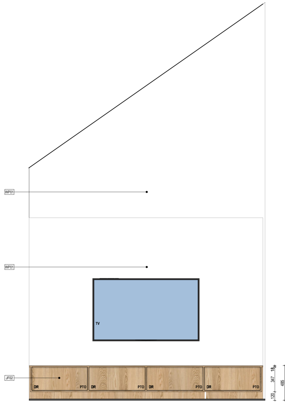
01 Living Elevation
